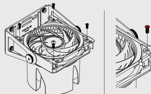
Screw installation without fan grill
