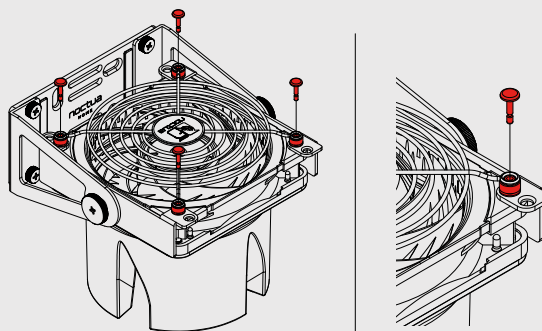
Push pin installation with fan grill
