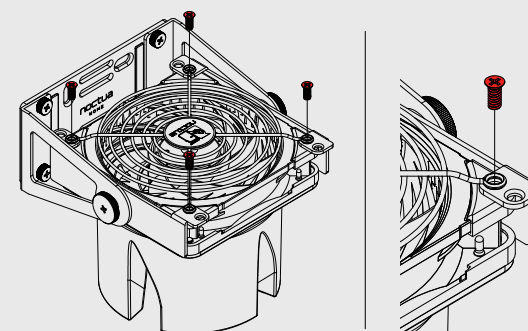
Screw installation with fan grill
