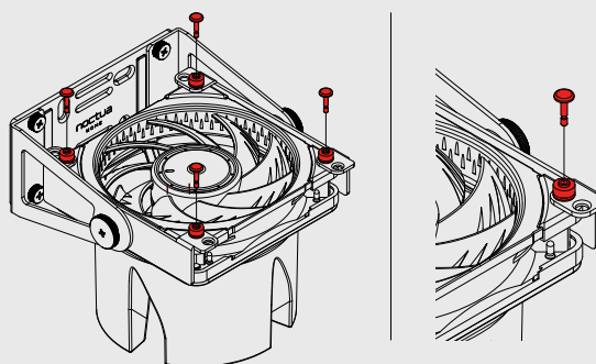
Push-pin installation without fan grill
