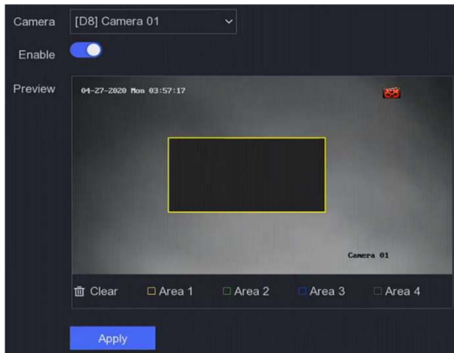
Figure 6-17 Privacy Mask
