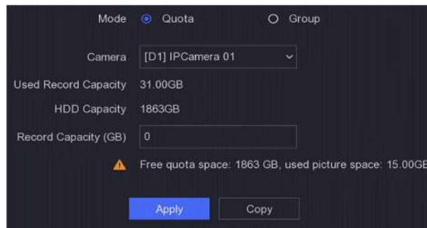
Figure 6-34 Quota
