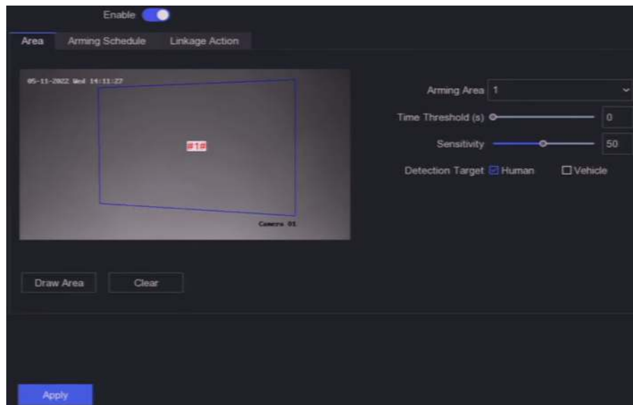
Figure 6-24 Intrusion Detection
