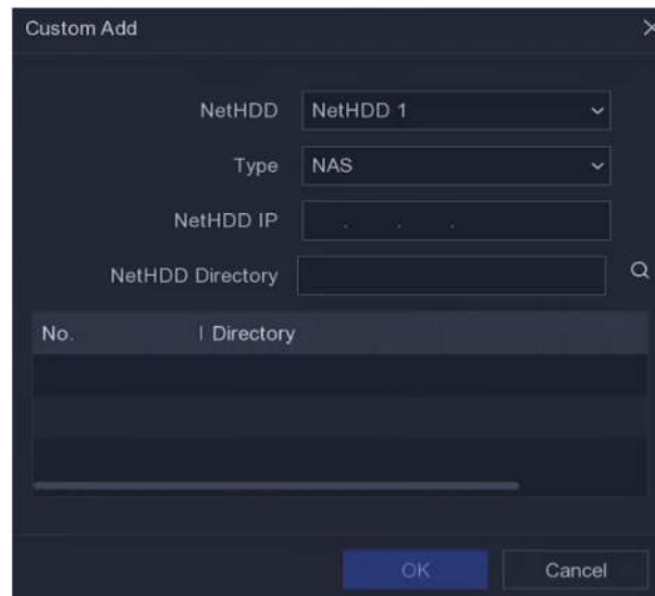
Figure 6-33 Add NetHDD
