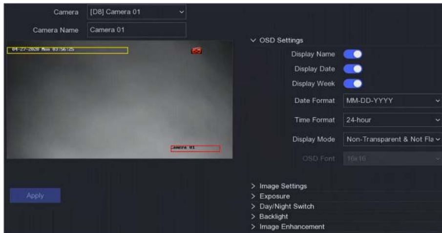
Figure 6-16 OSD
