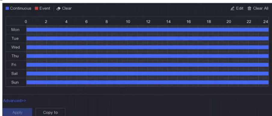
Figure 6-31 Recording Schedule
