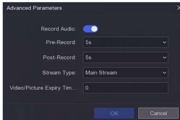
Figure 6-32 Advanced Parameters
