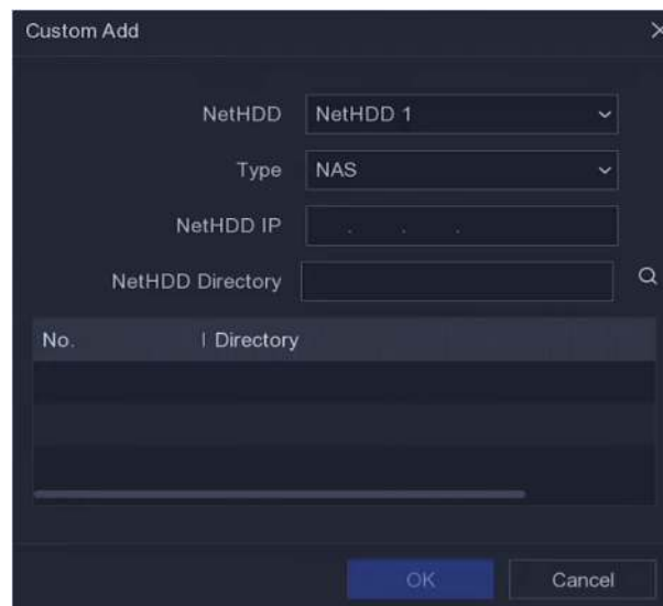
Figure 5-13 Add NetHDD
