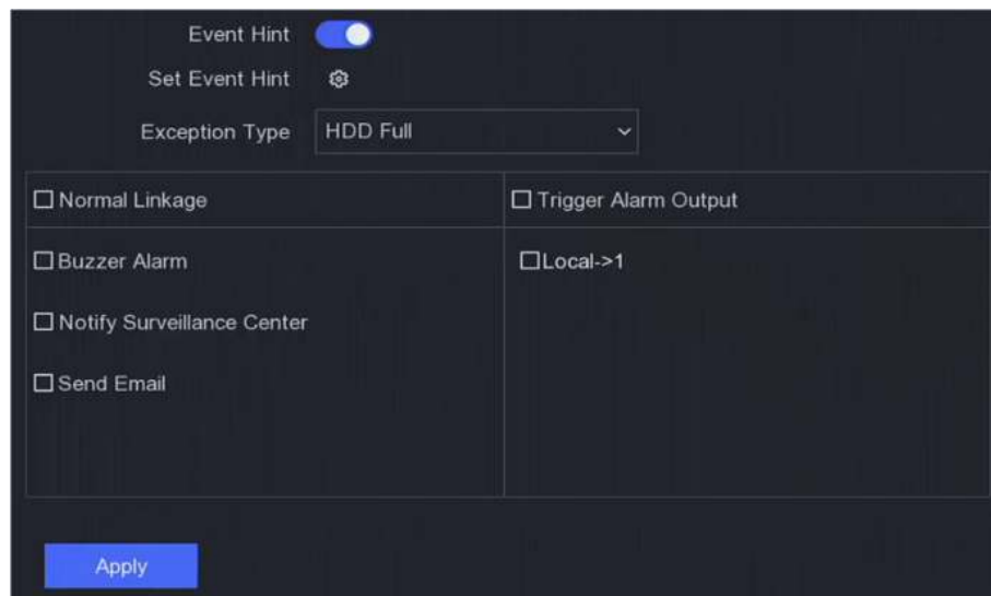
Figure 6-23 Exceptions
