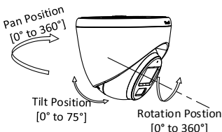
Figure 2-9 3-Axis Adjustment
