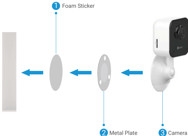
Fig.1 Mount by Foam Sticker
