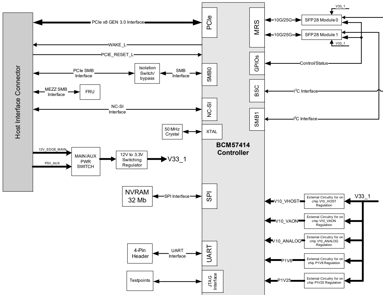
Figure 2: BCM957414M4142C Block Diagram
