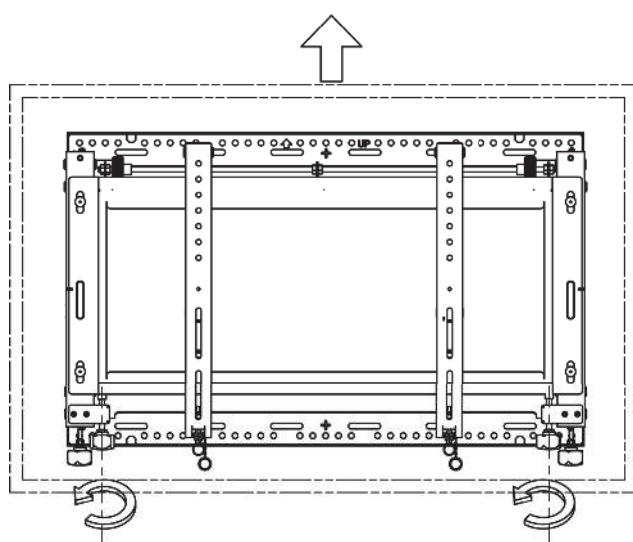
3. VERTICAL ADJUSTMENT
