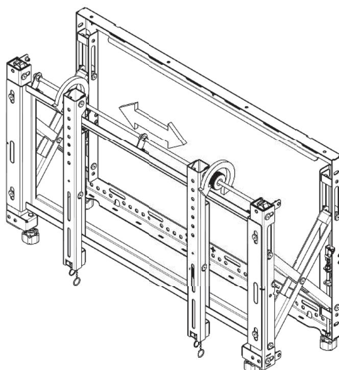
2. HORIZONTAL ADJUSTMENT
