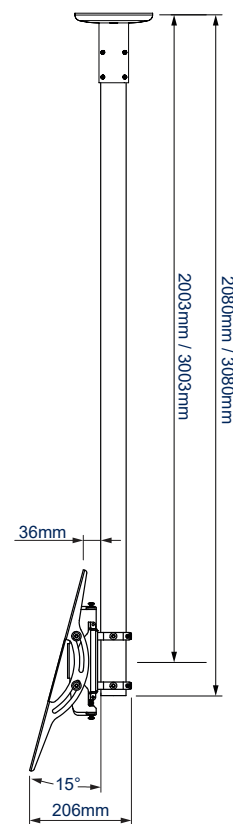
BT8424-200/300 SIDE VIEW - TILT UP
