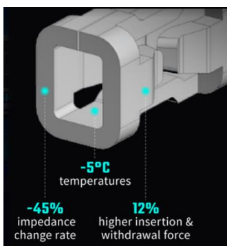
Enhanced 12+4PIN terminal structure
