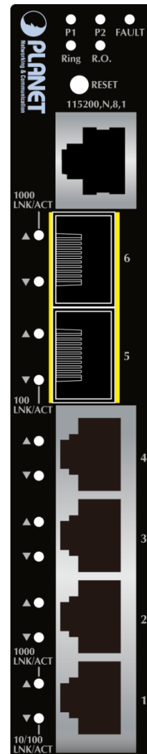
Figure 2-5: IGS-5225-4T2S Switch Front Panel
