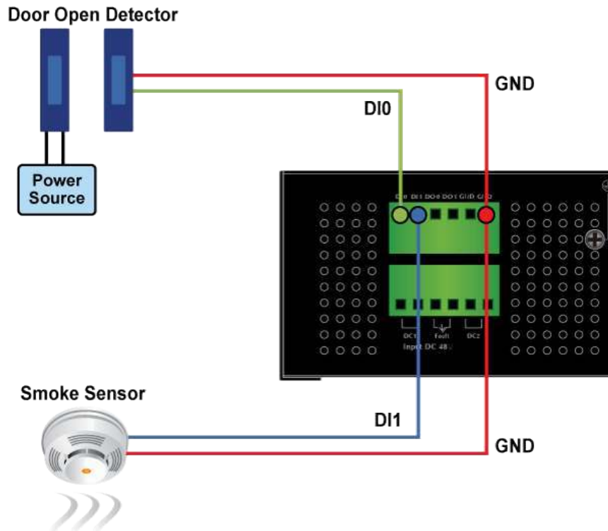
Figure 2-17 Wiring DI0 and DI1 to Open Detector
