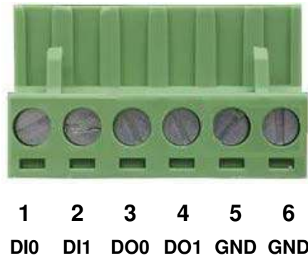
Figure 2-16 6-pin Terminal Block for DI and DO Wiring Input
