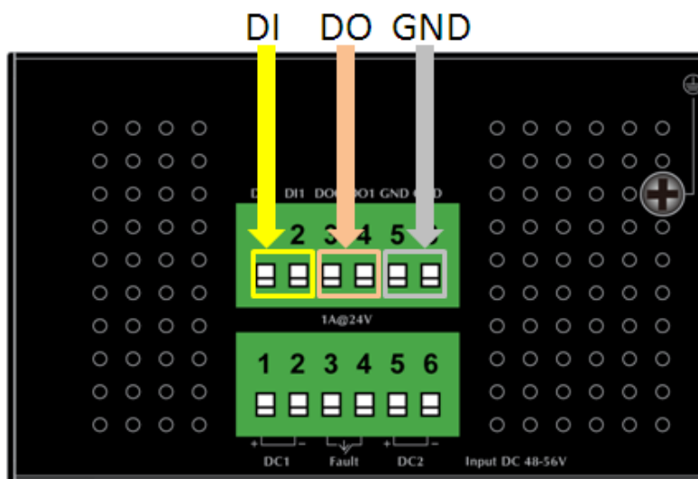
Figure 2-15 Wiring the Redundant Power Inputs
