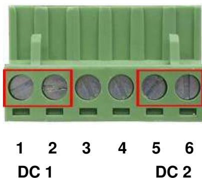
Figure 2-14 6-Pin Terminal Block Power Wiring Input
