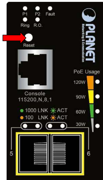
Figure 2-9 IGS-5225-4P2S Reset Button
