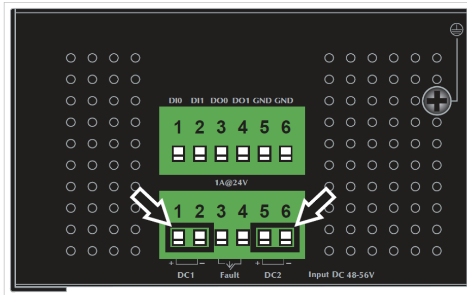
Figure 2-11: IGS-5225-8P2T2S and IGS-5225-8P4S Upper Panel
