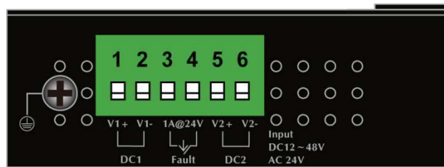
Figure 2-13: IGS-5225-4T2S Upper Panel
