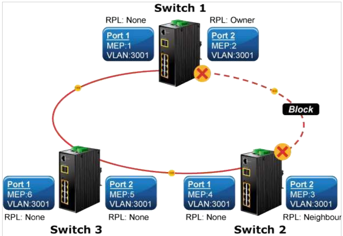
Figure 4-7-1-6: Ring Example Diagram
