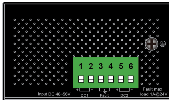
Figure 2-12: IGS-5225-4P2S Upper Panel
