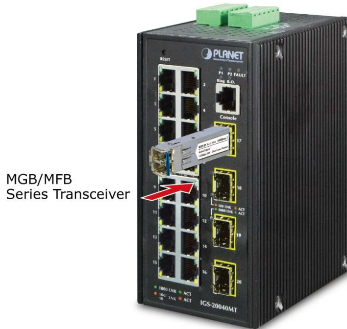
Figure 2-19: Plugging in the SFP/SFP+ Transceiver
