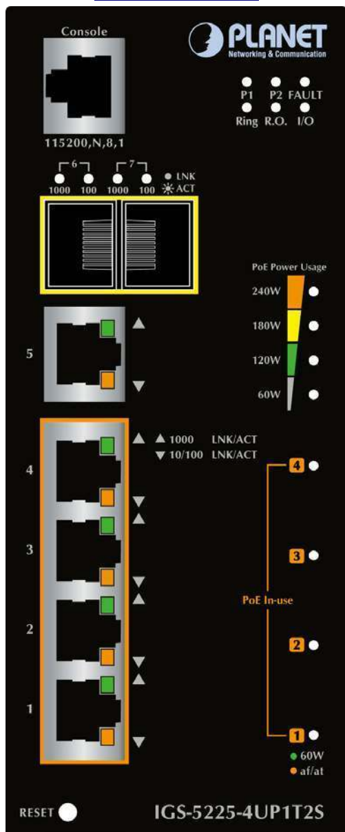
Figure 2-3: IGS-5225-4UP1T2S Switch Front Panel
