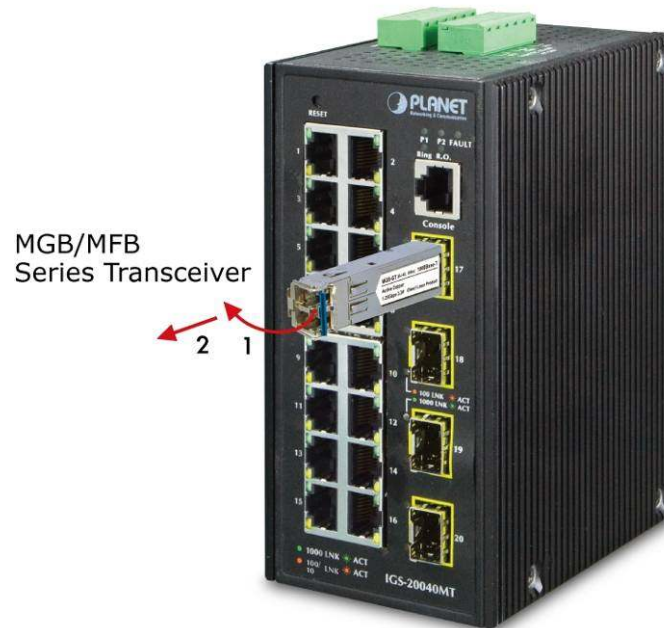
Figure 2-20: Pulling out the SFP/SFP+ Transceiver Module
