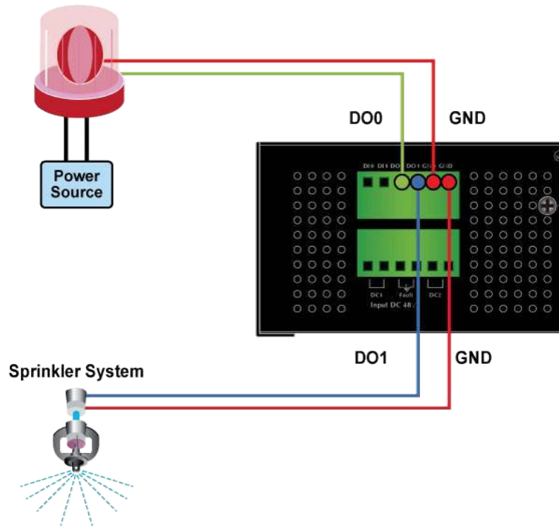
Figure 2-18 Wiring DO0 and DO1 to Open Detector
