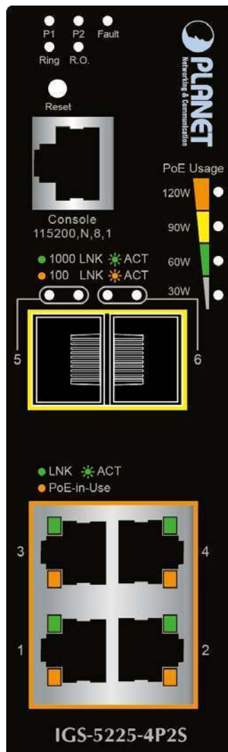
Figure 2-4: IGS-5225-4P2S Switch Front Panel
