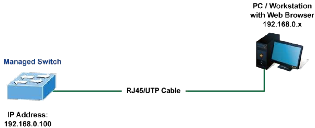
Figure 3-3: Web Management
