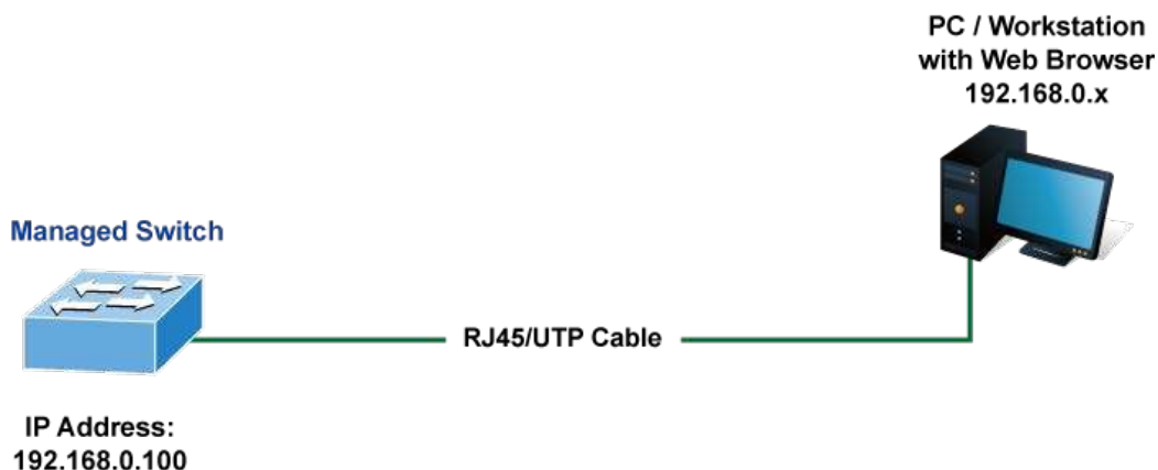
Figure 4-1-1: Web Management
