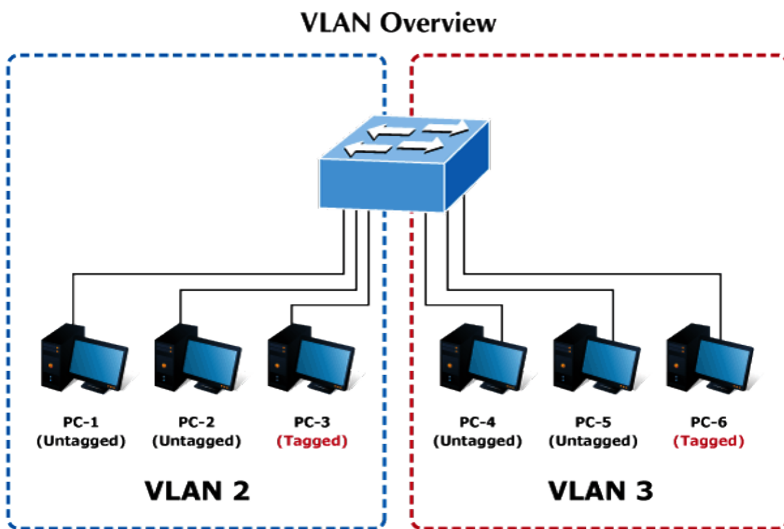
Figure 4-6-8: Two Separate VLANs Diagram
