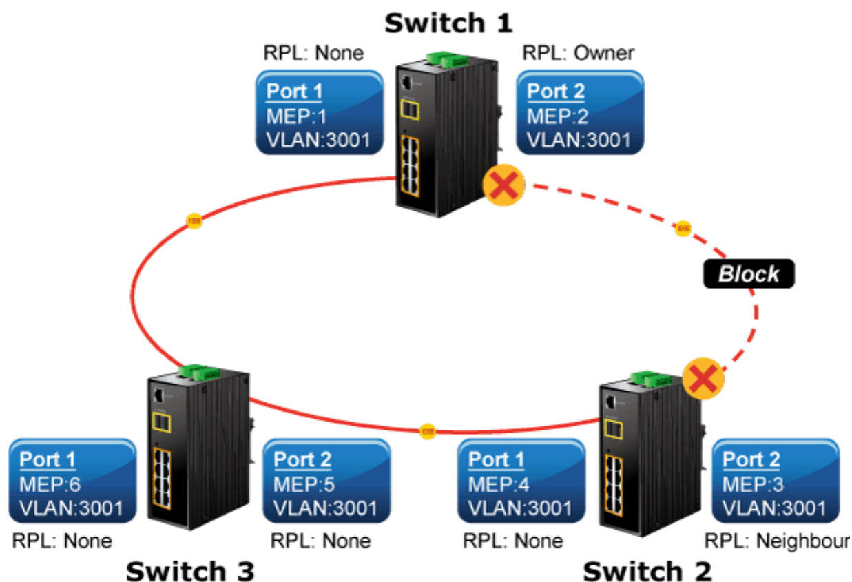
Figure 4-20-6: Ring Example Diagram
