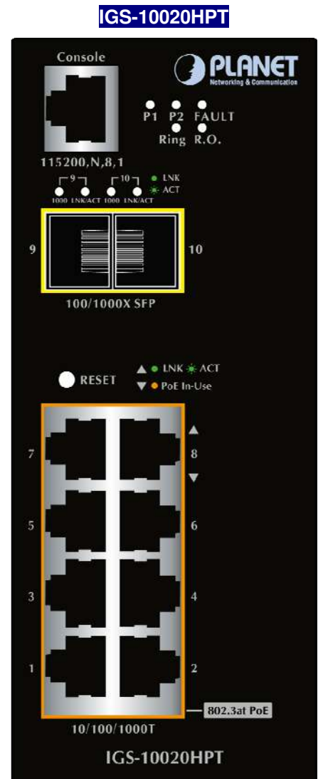
Figure 2-3: IGS-10020HPT Switch Front Panel
