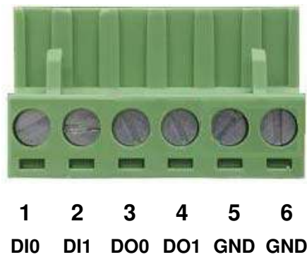
Figure 2-22 6-pin Terminal Block for DI and DO Wiring Input
