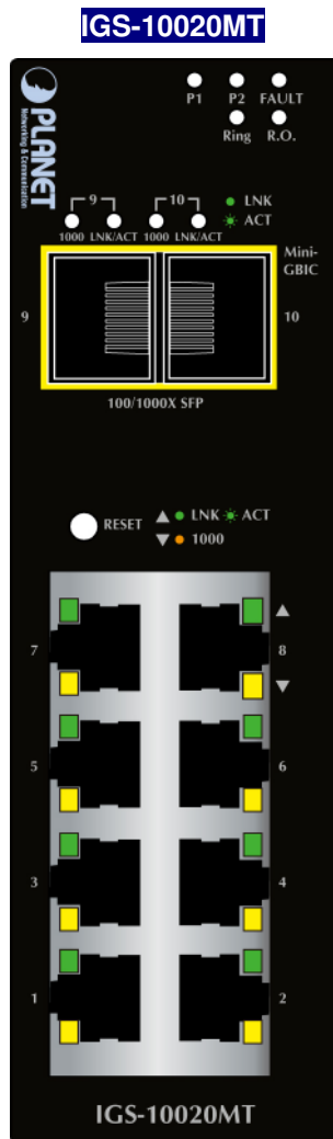
Figure 2-1: IGS-10020MT Switch Front Panel
