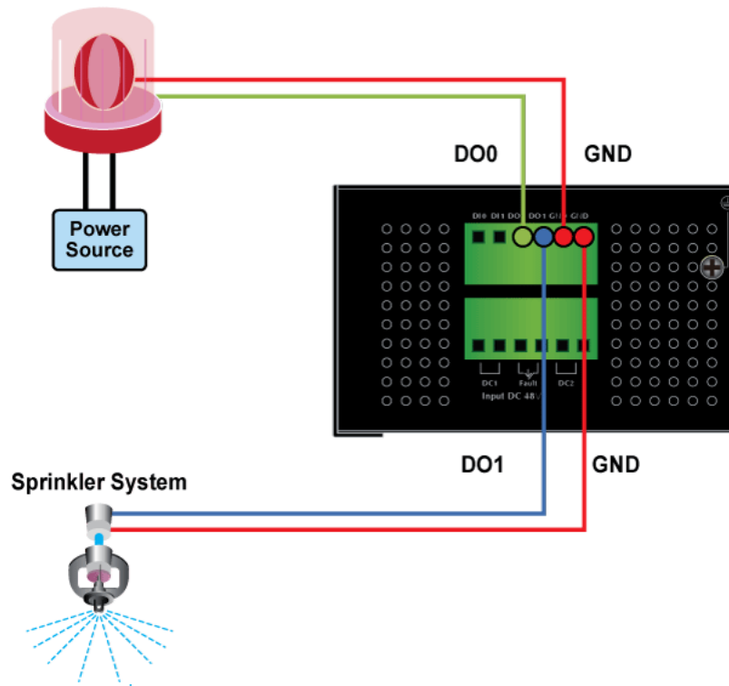
Figure 2-24 Wires DO0 and DO1 to Open Detector
