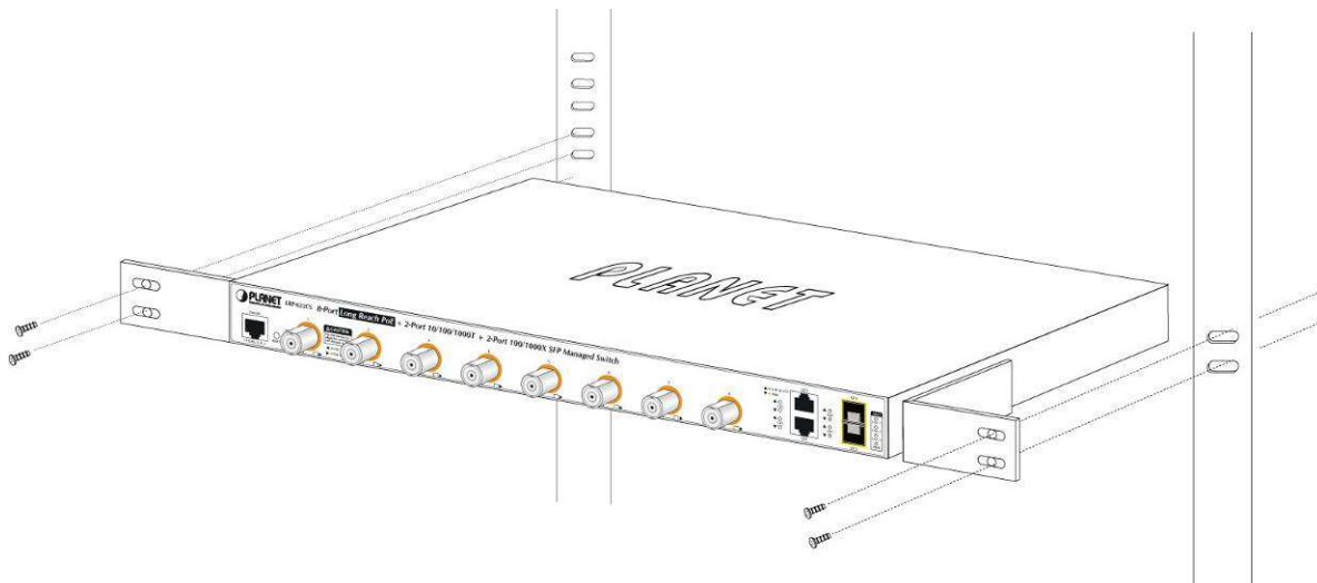
Figure 2-1-6 Mounting LRP Managed Switch in a Rack
