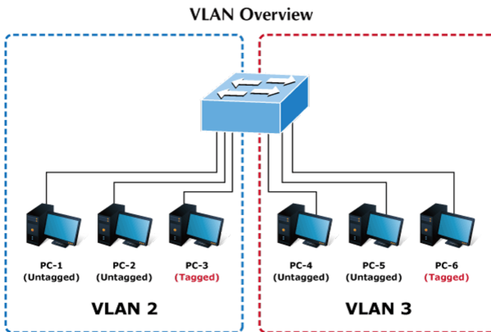
Figure 4-5-20 Two Separate VLAN Diagrams
