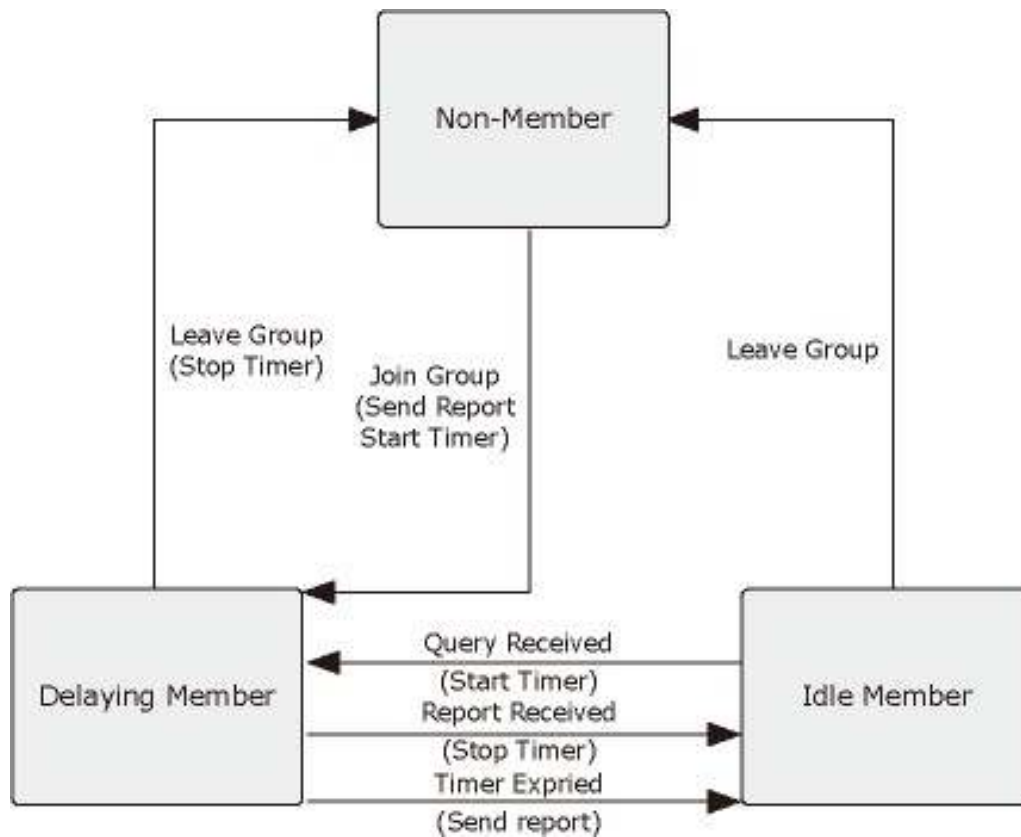
Figure 4-7-6 IGMP State Transitions
