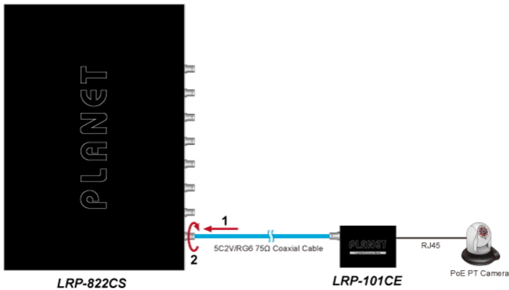
Figure 2-1-8 How to insert the coaxial cable from LRP Managed Switch
