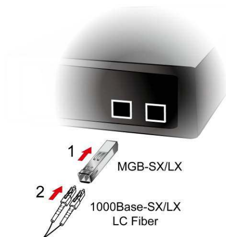
Figure 2-1-7 Plug in the SFP transceiver
