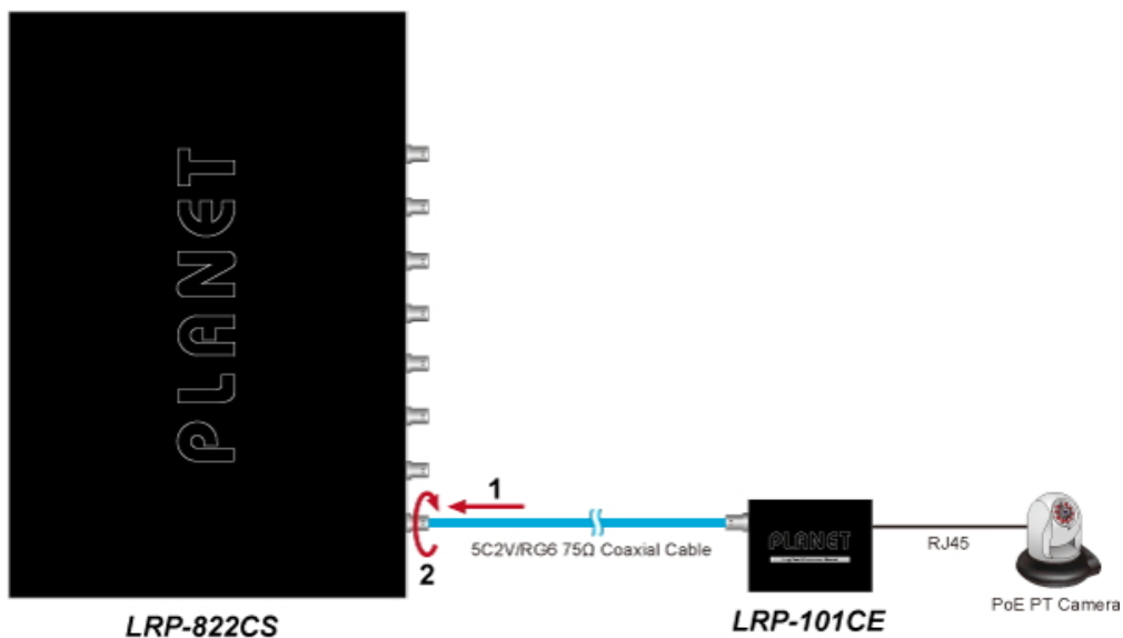
Figure 2-1-8 How to pull out the coaxial cable from LRP Managed Switch
