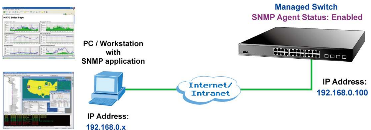
Figure 3-5: SNMP Management
