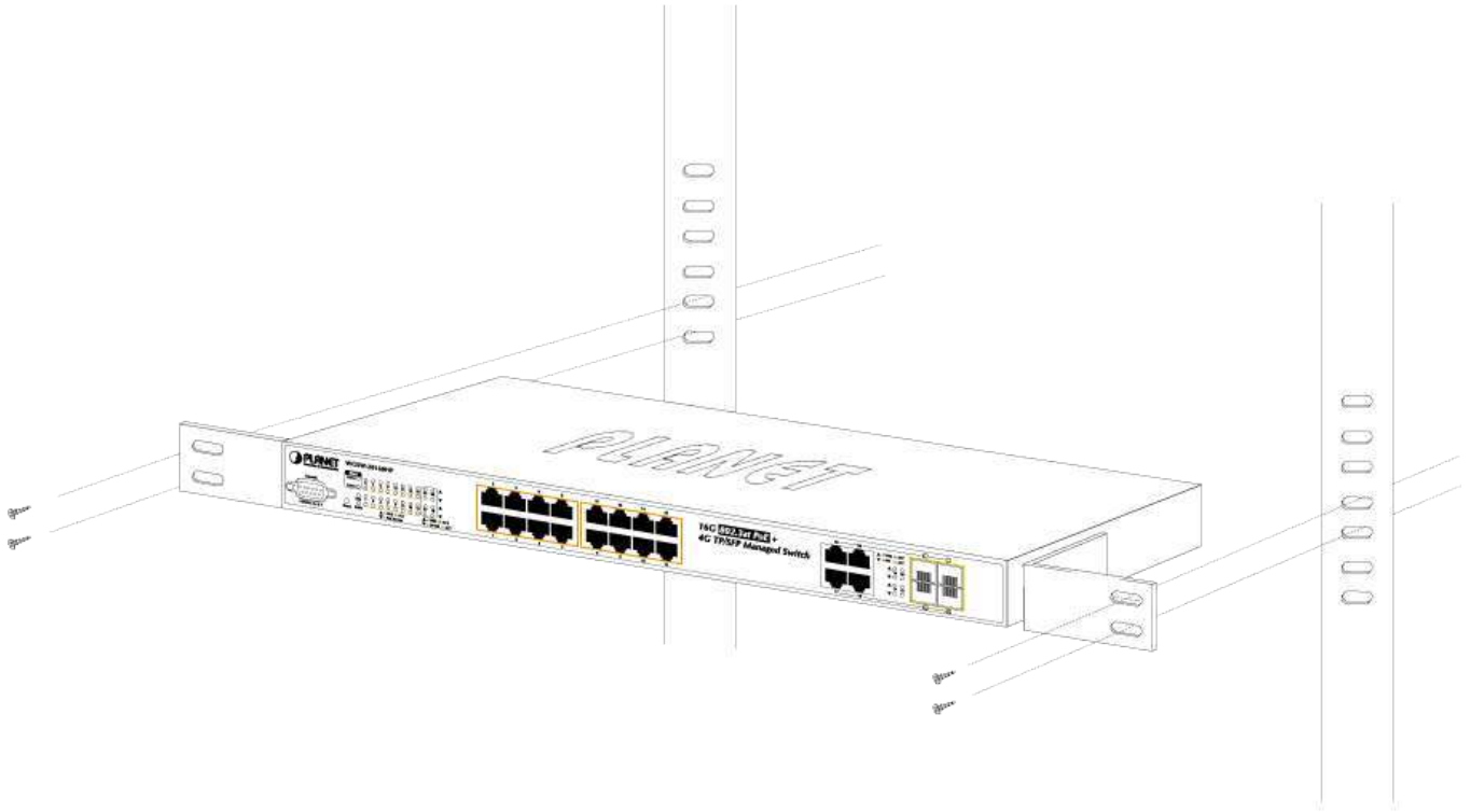
Figure 2-6: Mounting Managed Switch in a Rack
