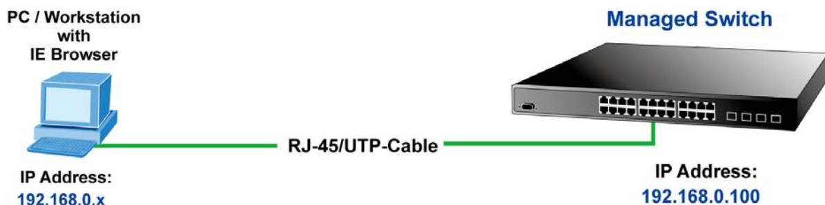
Figure 3-3: Web Management
