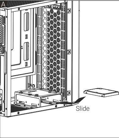
(5b) Install 2.5" SSD x 1
