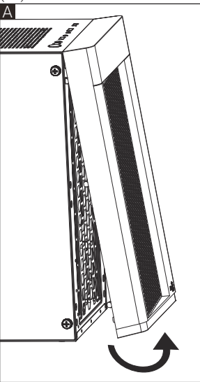
(7a) Install Front Radiator
