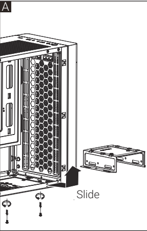
(5a) Install 2.5" SSD x 1
