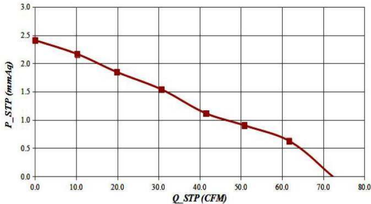
P-Q Curve
