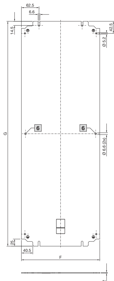
Mounting plate
