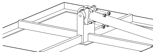
Fig. 4: Screwing the Nuts Hand-tight
