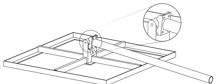
Fig. 2: Inserting the Mast
