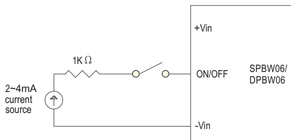
Application circuit
